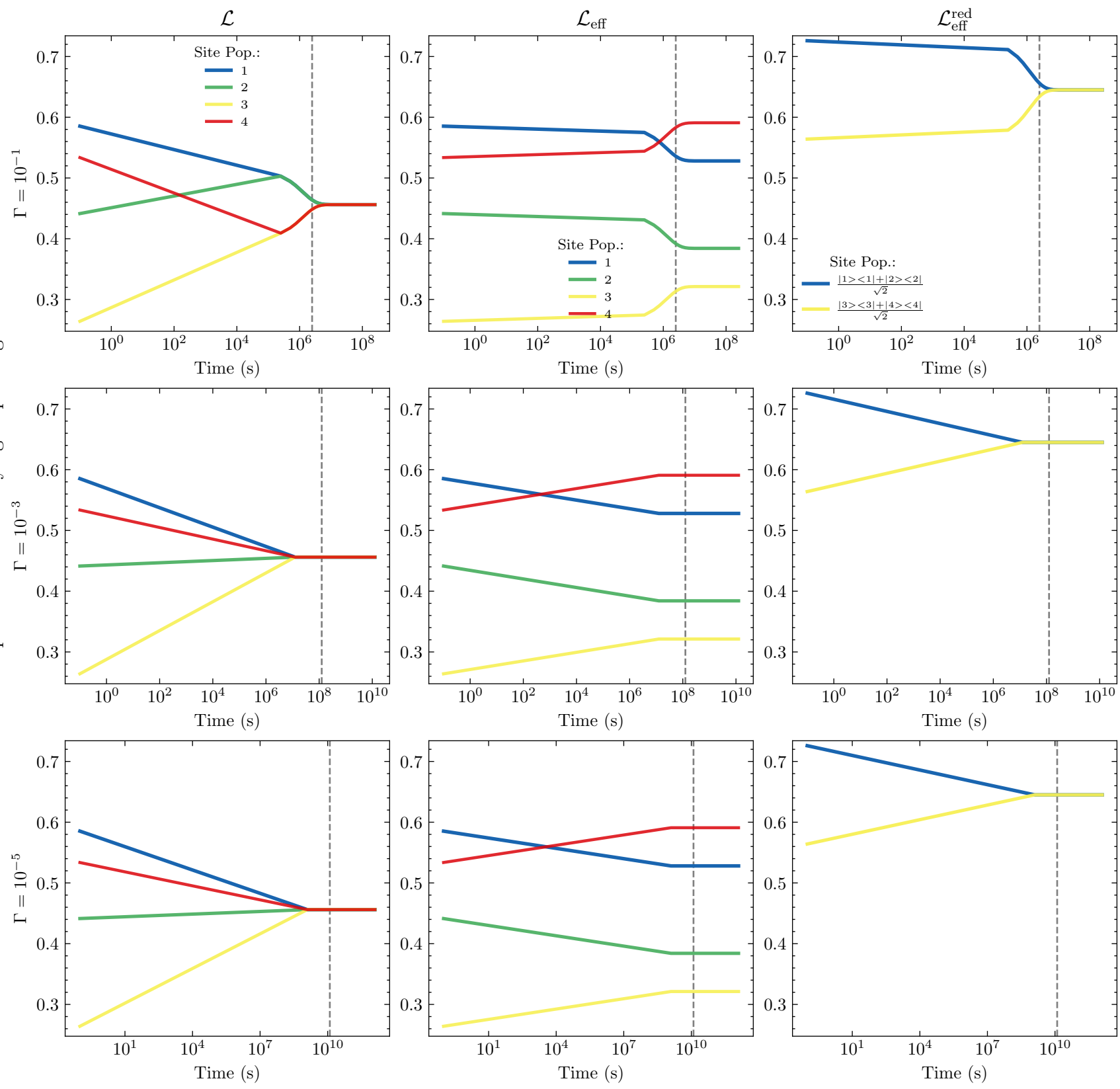
Time Evolution of Site Populations under \mathcal{L} , \mathcal{L}_{\text{eff}} , and \mathcal{L}_{\text{eff}}^{\text{red}} N=4 ; N_{\text{dimers}}=2 ; N_{\epsilon}=0 ; J = 10^{-1} ; \epsilon = 10^{-4} ; seed=381
